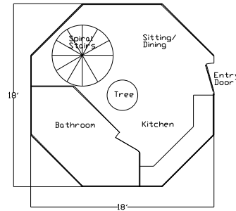
Two Story (example 1) 463 sq ft First Floor 272 sq ft
