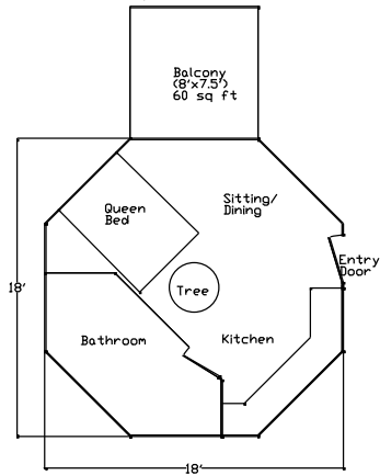
Single Story (example 1) 272 sq ft
