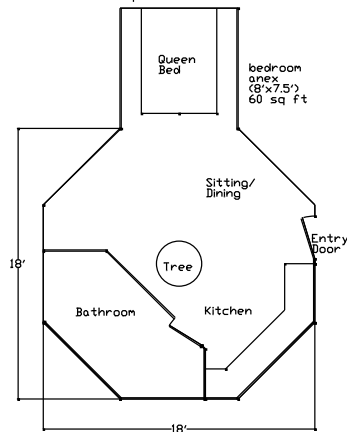
Single Story (example 2) 332 sq ft
